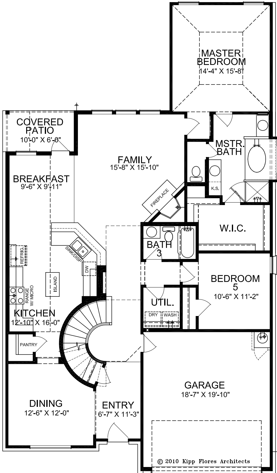
The Latour FIRST FLOOR
